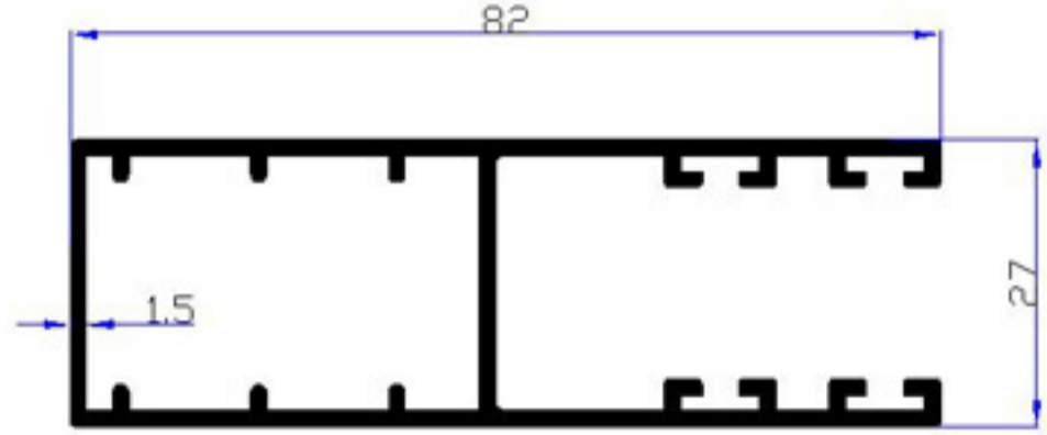
3632 - 1,075 kg/m
