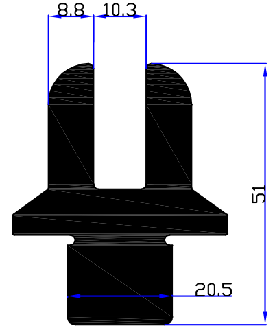
6653 - 2,967 kg/m
