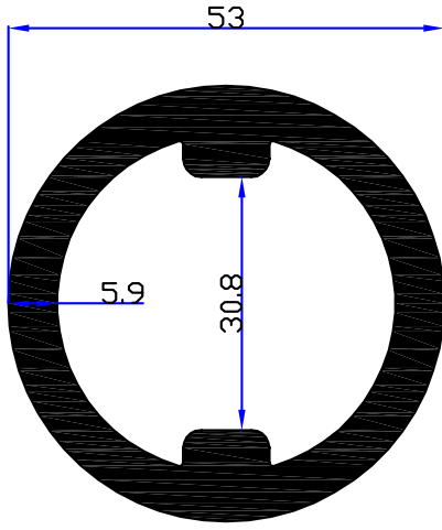
6651 - 2,625 kg/m
