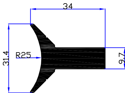
5393 - 1,005 kg/m
