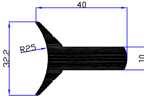
4711 - 1,175 kg/m
